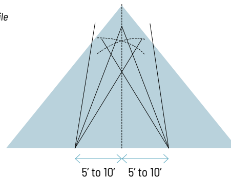
Drawing shown depicts the application of all tile profiles. Unless otherwise noted, it would apply to either concrete or clay tiles.
