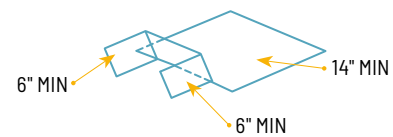
BACKER OR SADDLE FLASHING
