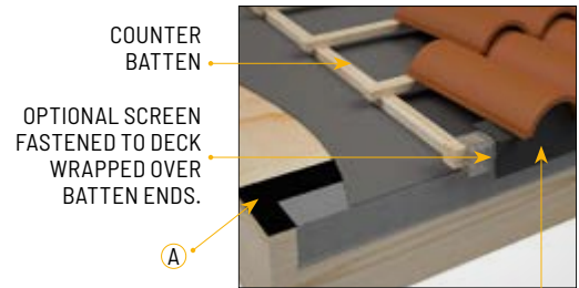
COVER METAL MIN 3/4" SPACE BETWEEN DRIP FLASHING & COVER METAL
